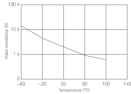
Figure 6. Typical video impedance variation with temperature
