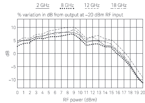
Figure 7. Typical square law deviation due to frequency
