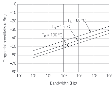
Figure 4. Typical tangential sensitivity
