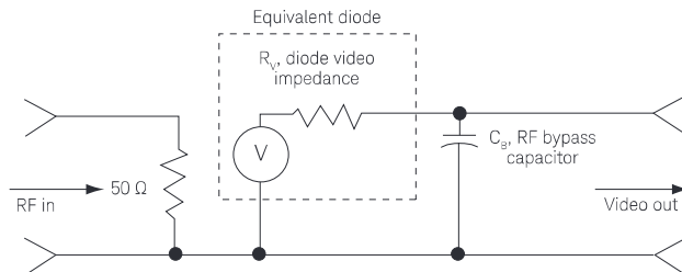
Figure 1. Equivalent circuit for 8474A/B/C/D/E with typical parameters
