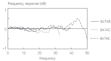
Figure 8. Typical frequency response
