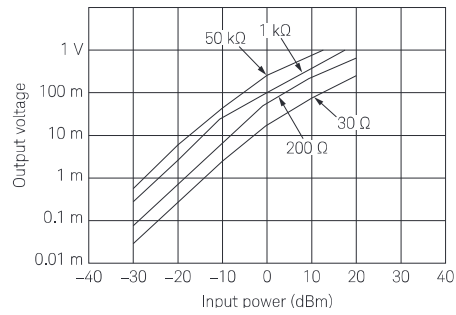
Figure 2. Typical transfer characteristics ( T_a = 25^\circ\text{C} )
