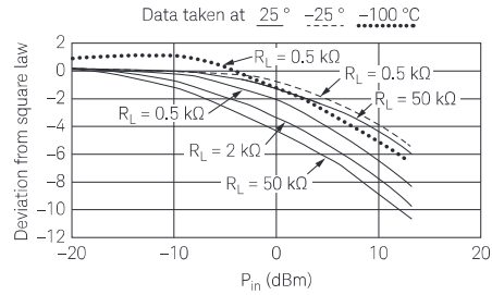
Figure 3. Typical square law deviation
